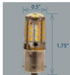
SLSCB250L Single Contact Bayonet LED; 2.5 Watts, 9 - 20 Volt operating range; 250 Lumen, Color Temp. 2750°K; IP67 Rated, 25,000 Hrs.
