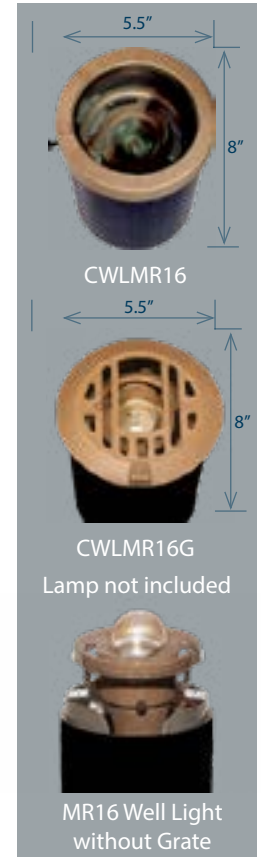
MR-16 Drop-In Well Light (CWLMR16 Series)
