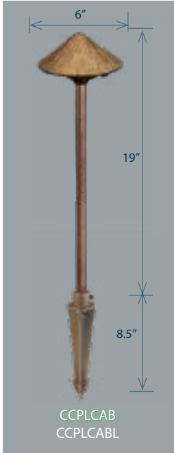
Craftsman-Cabana Path/Area Light (CCPLCAB) Integrated LED (CCPLCABL) Drop-In LED
