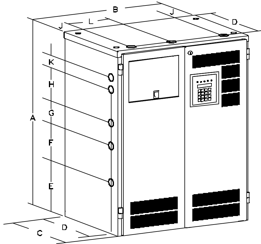
Figure 3.0 System Dimensions
