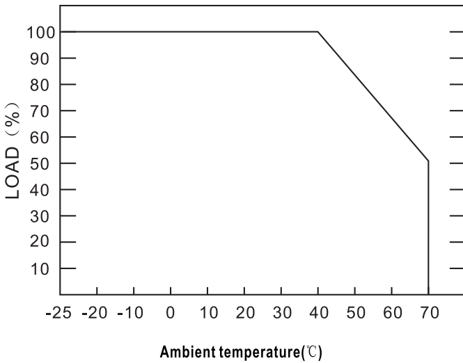
■ Derating Curve
