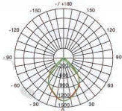
8 Inch AVERAGE BEAM(50%): 79.6
