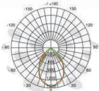
6 Inch AVERAGE BEAM(50%): 74.2
