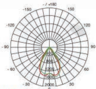
4 Inch AVERAGE BEAM(50%): 67.2
