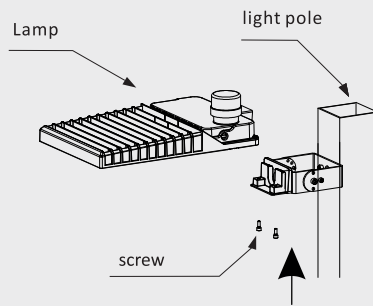
2. Install the light fixture on the lamp arm
