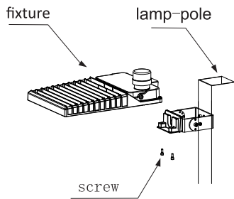
Install slip fitter on the lamp pole,wire and tighten screws
