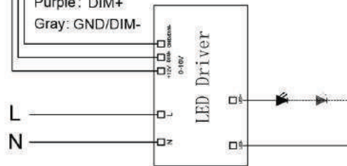
Wiring diagram
