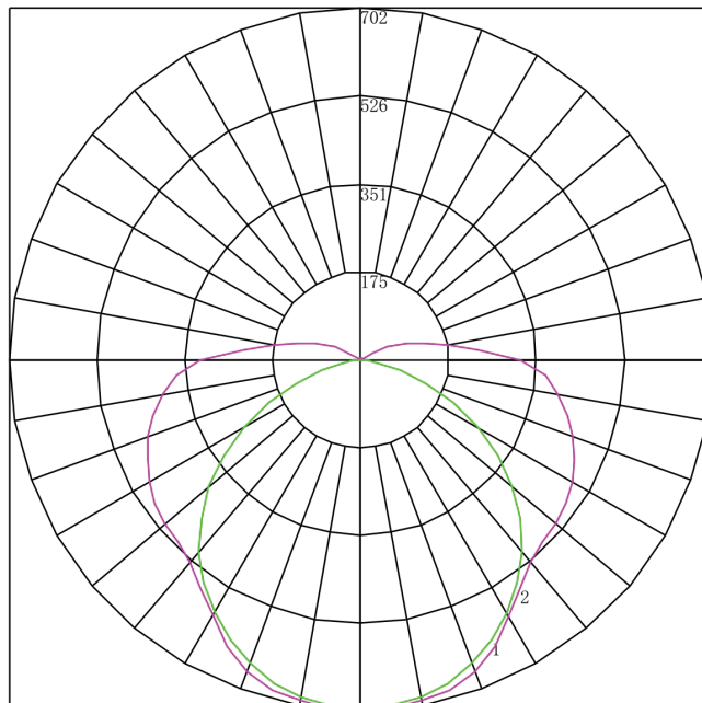
Maximum Candela = 701.568 Located At Horizontal Angle = 90, Vertical Angle = 5 # 1 - Vertical Plane Through Horizontal Angles (0 - 180) # 2 - Vertical Plane Through Horizontal Angles (90 - 270)
