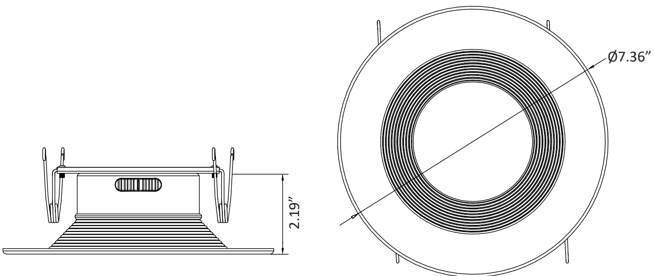
6 Inch Baffle
