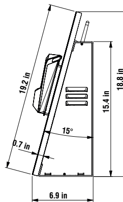
Variant Flex 21.5 lite incl. Magellan scanner, payment module and illuminated acrylic on top
