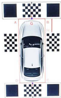
Placement standard: E, F are aligned with the vehicle center line, DC, AB are parallel with parameter filling: AD: calib length; DC: calib width; EG: front offset; BH: side offset
