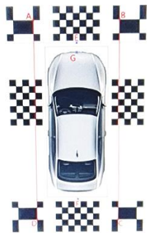
Pattern placement standard: E, F are aligned with the vehicle center line parameter filling: AD: left spacing; BC: right spacing; EG: front offset
