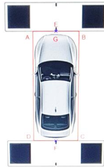
placement standard: E, F are aligned with the vehicle center line, DC, AB are parallel v parameter filling: AD: calib length; DC: calib width; EG: front offset
