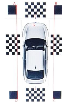
Pattern placement standard: E, F are aligned with the vehicle center line parameter filling: AD: left spacing; BC: right spacing; EG: front offset
