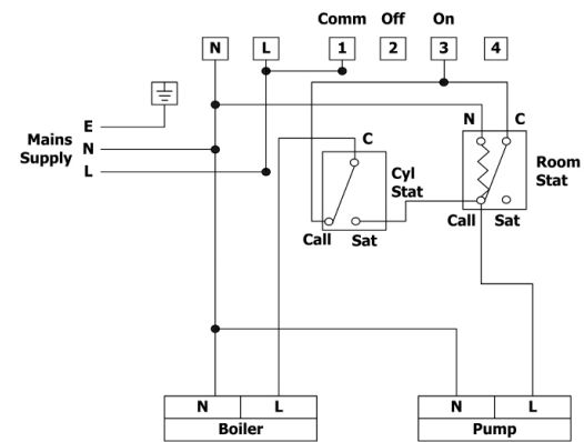
3. Gravity primary with pumped Heating via RoomStat and CylinderStat
