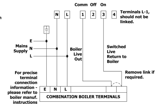
4. Typical combination boiler installation
