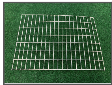
1" x 1/2" 16 gauge
