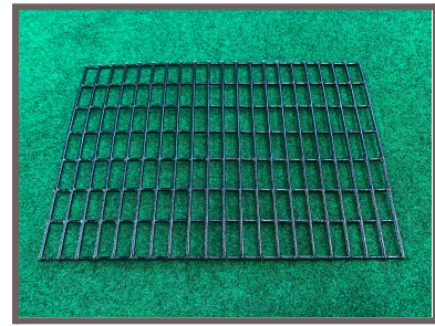
1" x 1/2" 16 gauge
