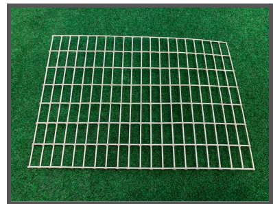
1" x 1/2" 16 gauge
