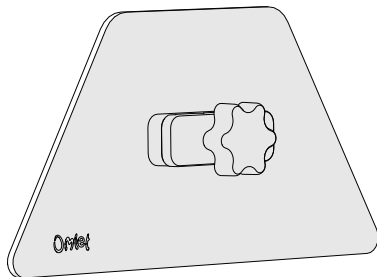
Geo60 Mirror Assembly Half Hexagon 052.0089 x1
