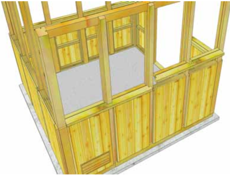
Outside Angle Cut Polygal Window
