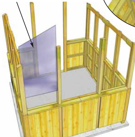
Outside Angle Cut Polygal Window
