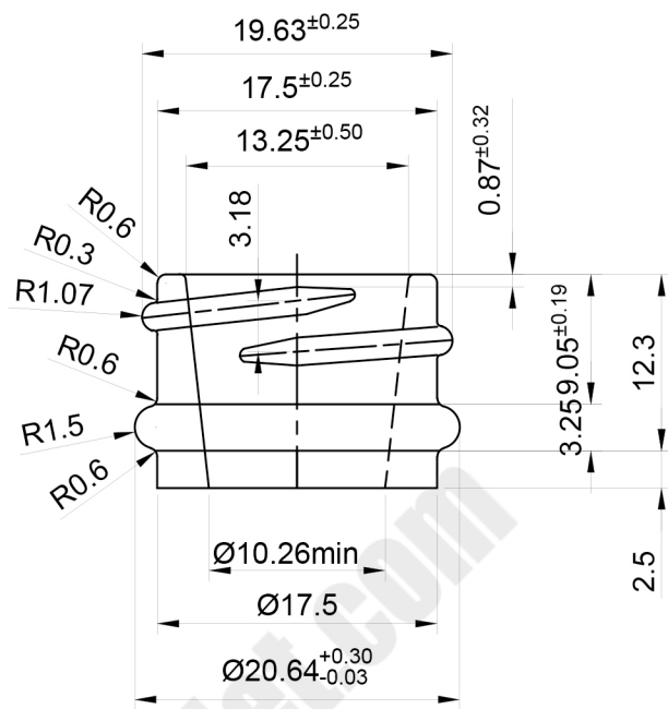
NECK FINISH DETAILS SCALE -2:1
