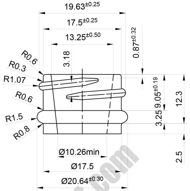
NECK FINISH DETAILS SCALE -2:1
