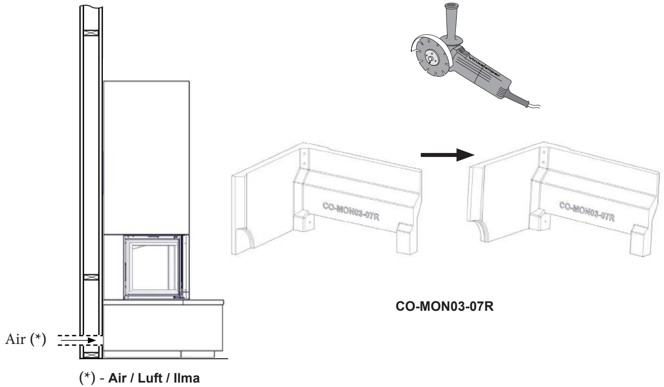
FIG 4 Monaco A Low Base_Q-34 AL + Bench
