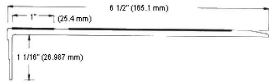
Type 365 6 1/2" wide, 5/32" thick, nose 1 1/16" underside, beveled back
