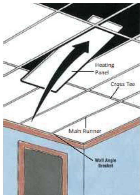
Figure 6b – Placing in Ceiling Grid
