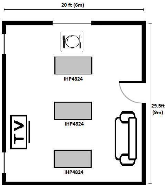
Figure 9c – Large Room Installation Plan View
