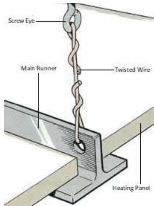
Figure 6a – Close-up of T Bar Support
