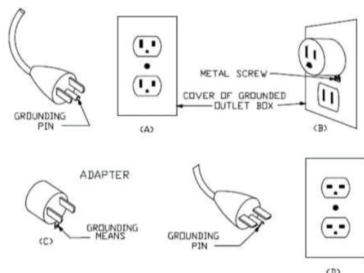
Figure 5b – Grounding Adapter Plug
