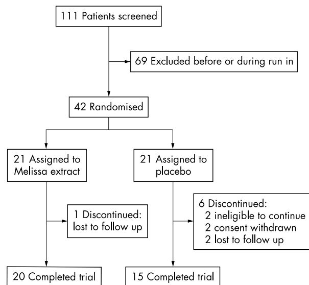
Figure 1 Trial profile.
