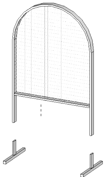
EXPLODED VIEW
