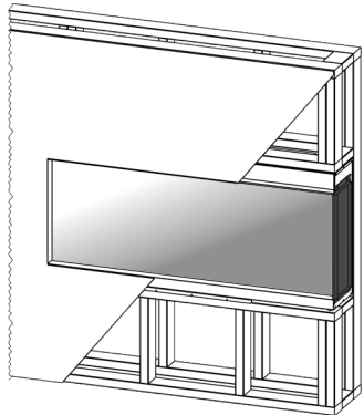
FINISHED WALL - RIGHT CORNER INSTALL
