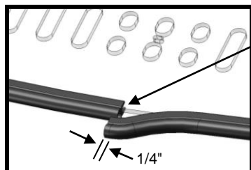
Co-extruded bulb seal starting/finishing point
