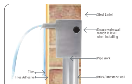
Installation suggestion
