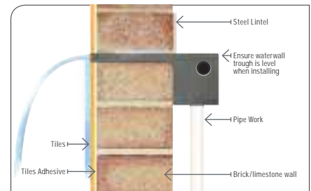
Installation suggestion
