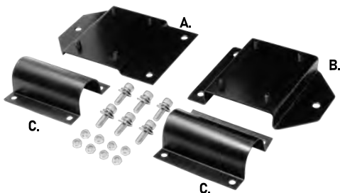
(2) HEAVY DUTY MOUNTING BRACKETS: Includes: A. (1) HEAVY-DUTY FLAT MOUNTING PLATE B. (1) HEAVY-DUTY DEEP MOUNTING PLATE C. (2) HEAVY-DUTY FRAME TUBE CLAMPS (1) MOUNTING HARDWARE
