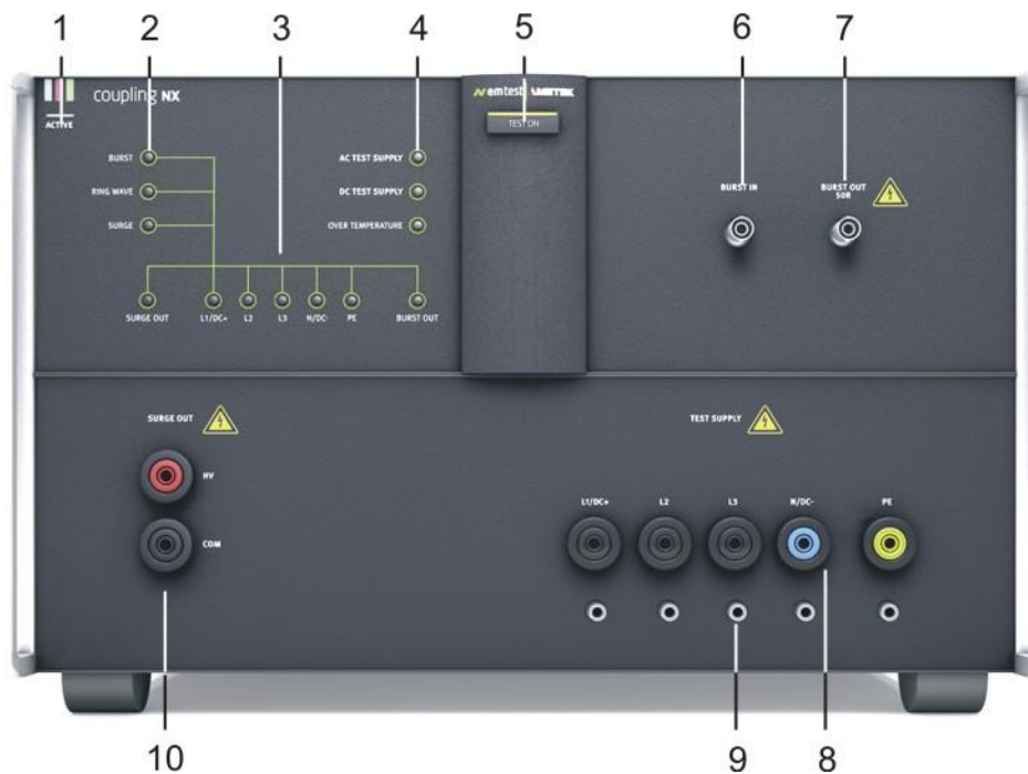
Figure 5.1: coupling NX front side ( model for 5kV/16 A / 32 A )
