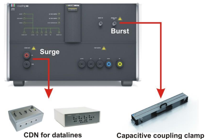
Figure 6.1: External device plug for Burst and Surge
