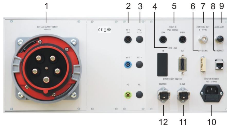
Figure 5.4: coupling NX front view (model for 5kV/100 A / 16 A)
