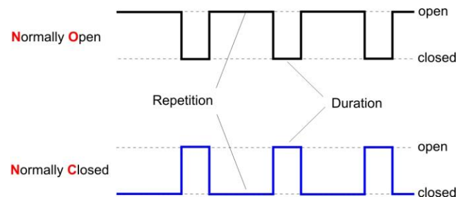
Figure 3.2. : Operating modes Switch BS 200N100
