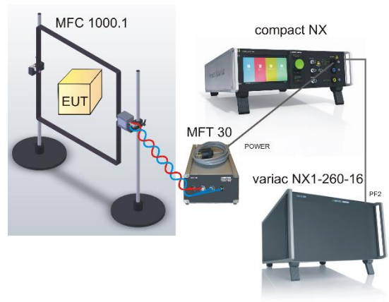
Test setup
