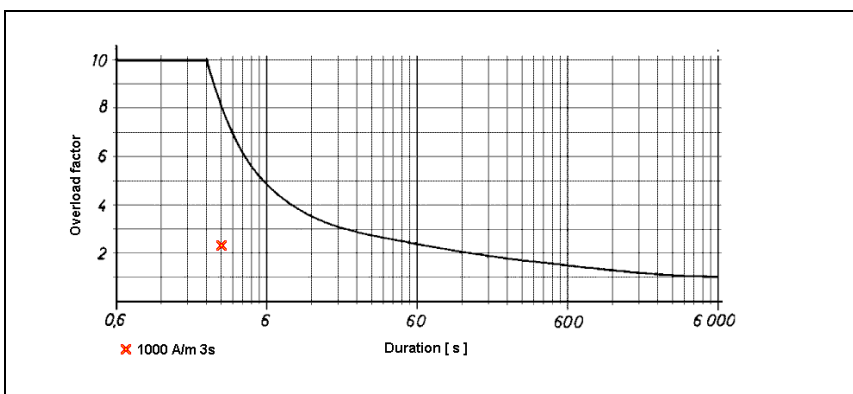
Load diagram variac NX1-260-16
