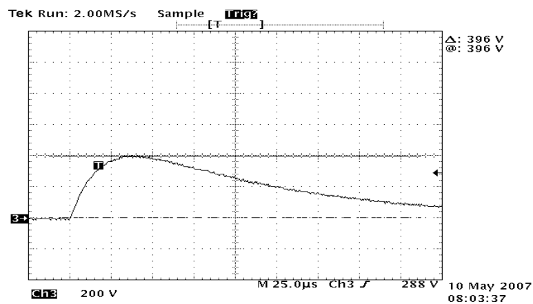
Generator source impedance verification
