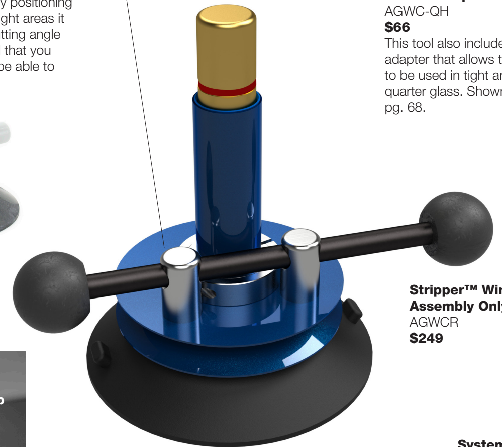
Precision Machined Components The Stripper™ winding hub was designed and manufactured using 6061 aluminum with a hardened anodized finish. The tools small diameter hub allows for maximum torque when cutting.
