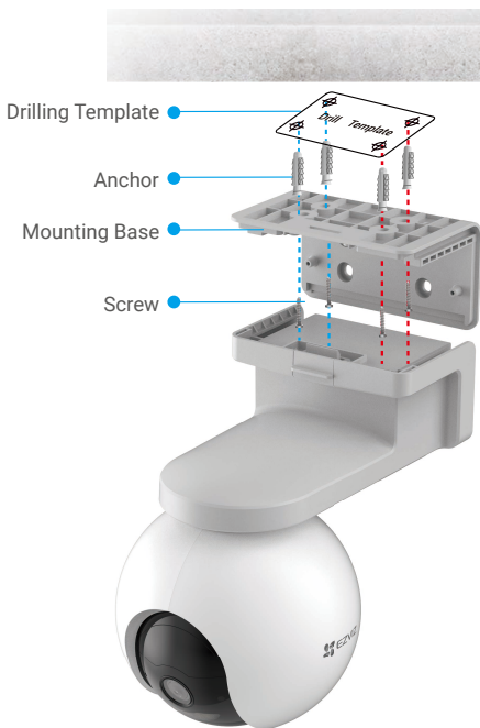
Fig. 1 Ceiling Mount
