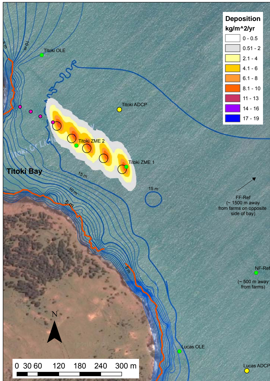
Figure 3. Proposed sampling stations, bathymetry, reef extent and depositional footprint at the Akaroa Salmon Titoki Bay farm. The circular pen layout is shown at each farm. Proposed standard sampling stations are in green, sampling stations along a transect towards the nearshore reef habitat are in pink, and ADCP locations are in yellow. The red line shows the reef extent. Predicted depositional footprints were modelled under a 'no-resuspension' scenario, with a feed loading of 0.5 kT yr -1 . The OLE (200 m from the farms) and the FF-Ref (~1500 m from the farms) positions are indicative only and the specific locations will be determined during sampling to ensure that the stations are similar in depth, proximity to shore and sediment characteristics.
