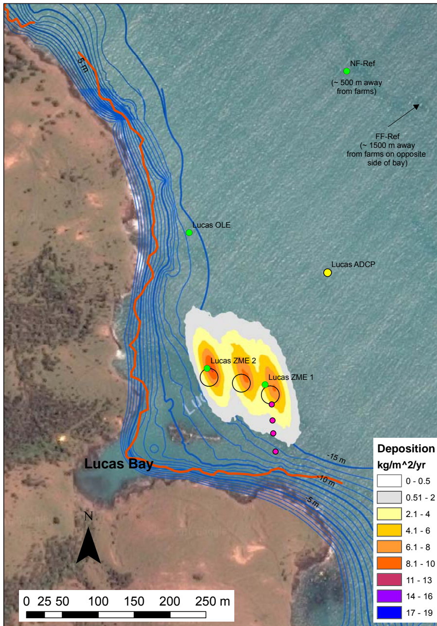
Figure 4. Proposed sampling stations, bathymetry, reef extent and depositional footprint at the Akaroa Salmon Lucas Bay farm. The circular pen layout is shown at each farm. Proposed standard sampling stations are in green, sampling stations along a transect towards the nearshore reef habitat are in pink, and ADCP location is in yellow. The red line shows the reef extent. Predicted depositional footprints were modelled under a ‘no-resuspension’ scenario, with a feed loading of 0.4 kT yr -1 . The OLE (200 m from the farms) and the FF-Ref (~1500 m from the farms) positions are indicative only and the specific locations will be determined during sampling to ensure that the stations are similar in depth, proximity to shore and sediment characteristics.
