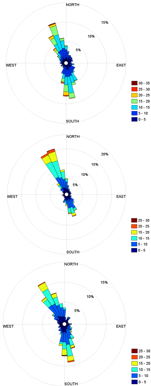
Figure A2-1. Mean current speed and direction measured at surface (0 m depth), mid-water (7 m above seabed) and near-seabed (3 m above seabed) at the Titoki Site.
