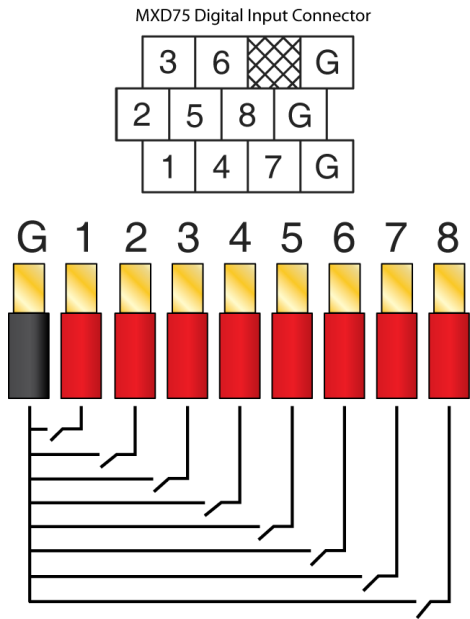
MXD75 Surface Mount Instrument Digital Inputs Connection Detail.
