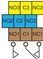
MXD75 Relays 1 - 3 Connector
