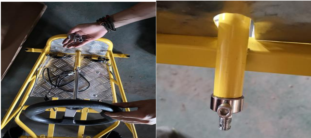
7. Install tie rod to front frame.
