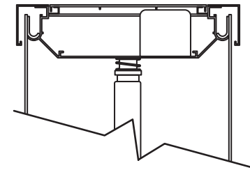
A Illuminated Cabinet • Typical Section Scale 1 1/2" = 1' For Production
