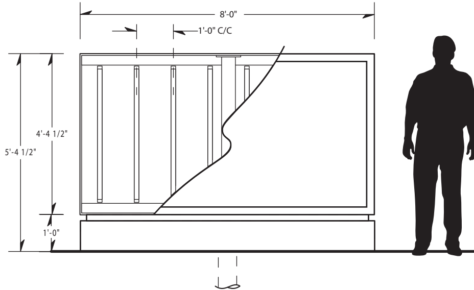
A D.F. Illuminated Pole Sign • Cabinet Detail Scale 3/8" = 1' For Production
