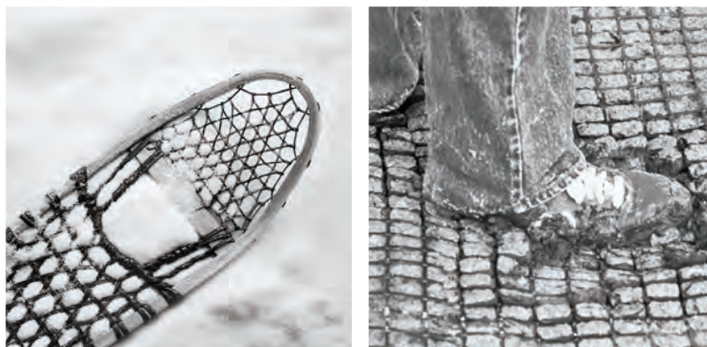
Image 1: The Snowshoe Effect – Tensor TriAx and BX Geogrids distribute heavy loads over soft soils just like a snowshoe supports the weight of a man over soft snow.
