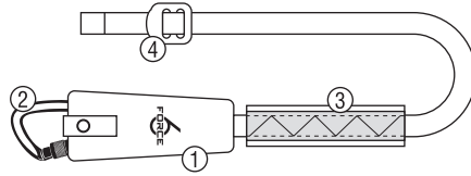
1 - Carabiner Pouch | 2 - Carabiner | 3 - Shoulder Webbing Stabilizer 4 - Triglide Buckle
