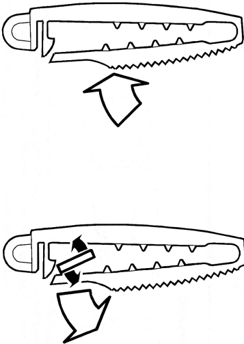
Unlocking clip with screwdriver
