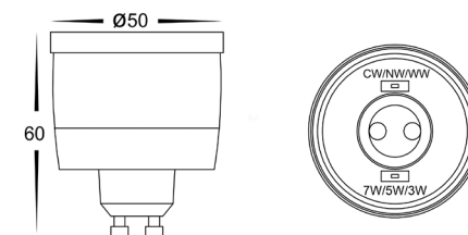
HV9507 + HV9508 Dimensions
