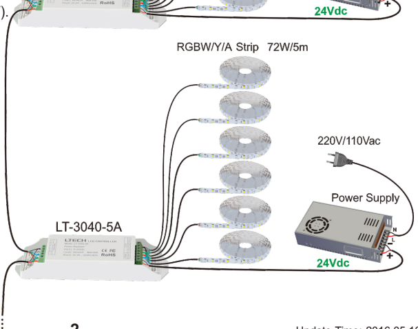
B. 24V lamp connected, loads 0~480W(24V).
