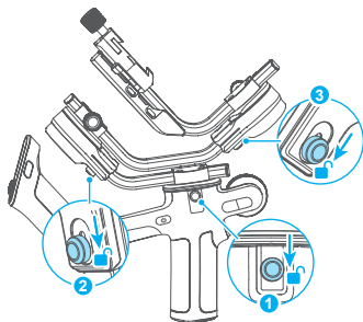
Gimbal folded position
