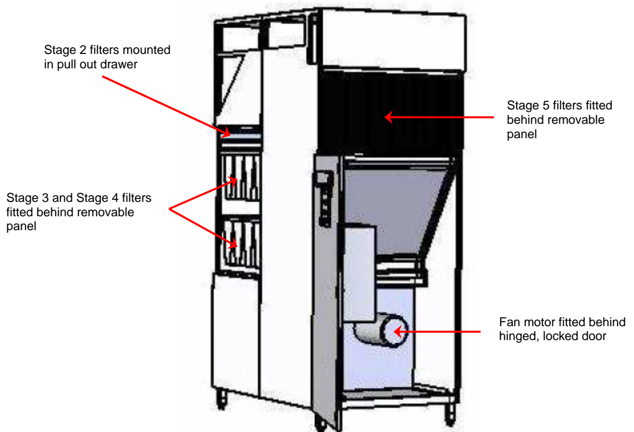
Refresh Ultima Services Tower Showing the Location of Filter Stages 2 to 5
