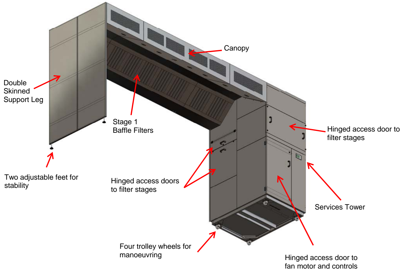
Overview of Overview of Refresh Ultima Unit
