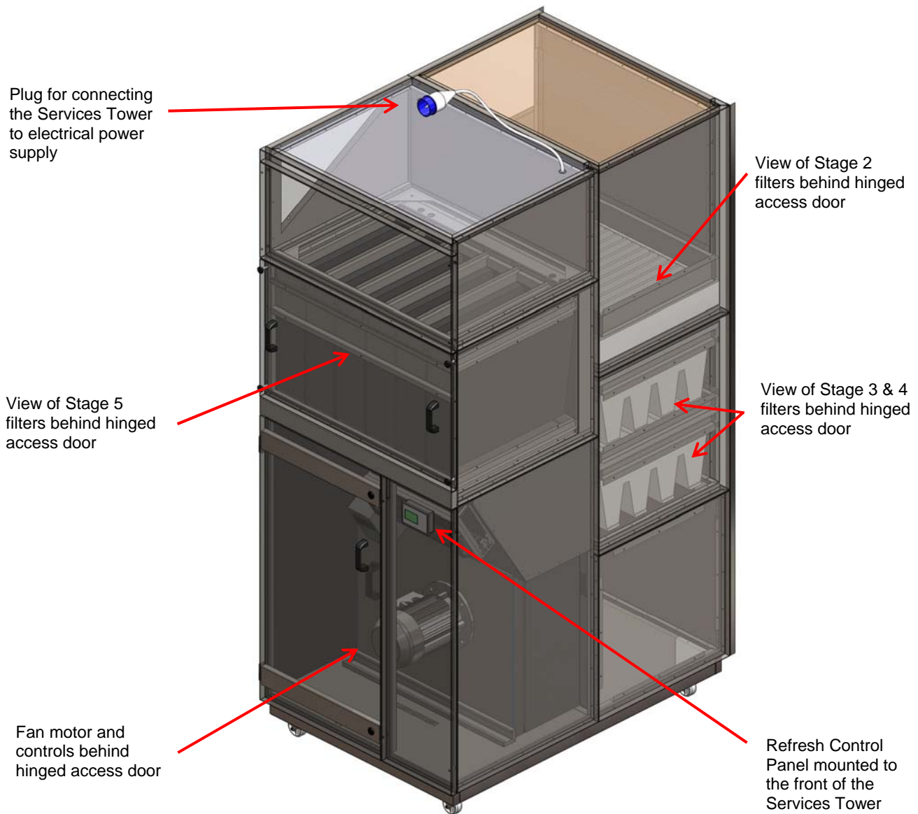
Overview of Refresh Ultima Unit Services Tower
