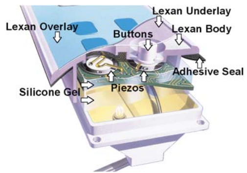
Panel Construction
