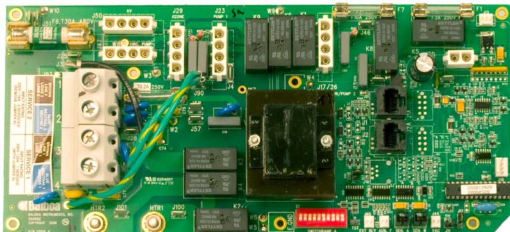
GS500Z Board
