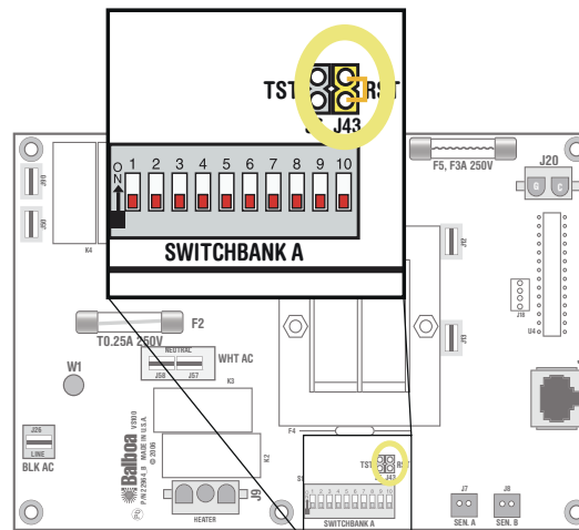
J43 on VS100/GS100 Series Main Board Shown.
