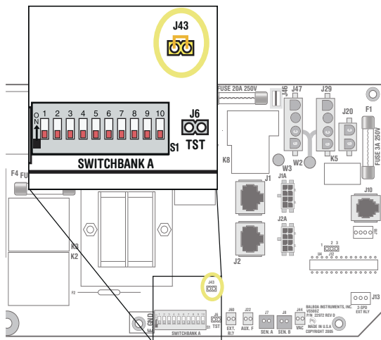
J43 on VS5xxZ and VS300 Series Main Board Shown. J43 on GS5xxZ Series is located in approximately the same position.
