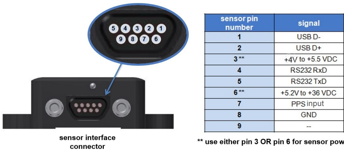
Figure 37 -Connector Wiring
