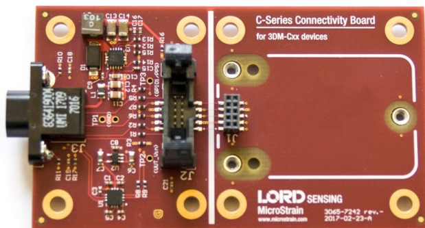
Figure 40 -C-Series Connectivity Board
