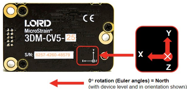
Figure 19 -Sensor Frame
