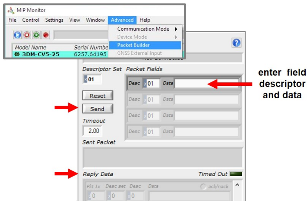
Figure 35 -Packet Builder
