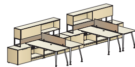
pedestal supported desks with technology credenzas and freestanding overheads overall dimensions 240"W 82.5"D 56"H
