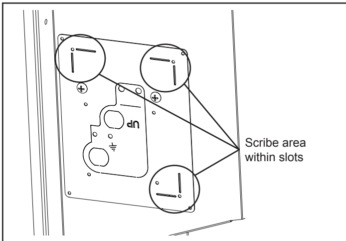
Figure 6 - Scribe slots
